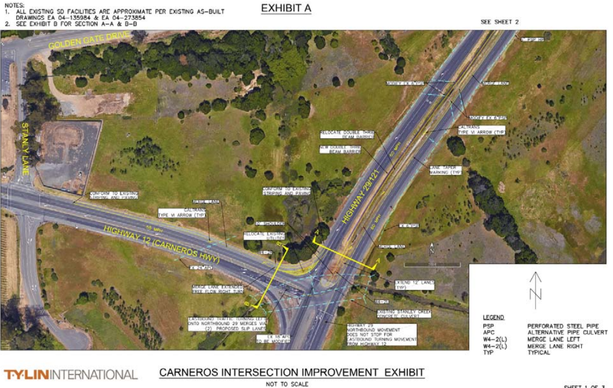
Figure 29: Carneros Junction Intersection Improvements
